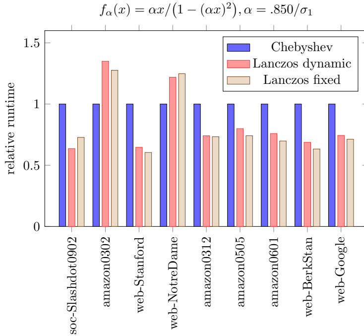
FIG. 6. Plot of relative runtimes for approximating f_\alpha^\circ(B)w , \alpha = .850/\sigma_1 , using the three methods.
